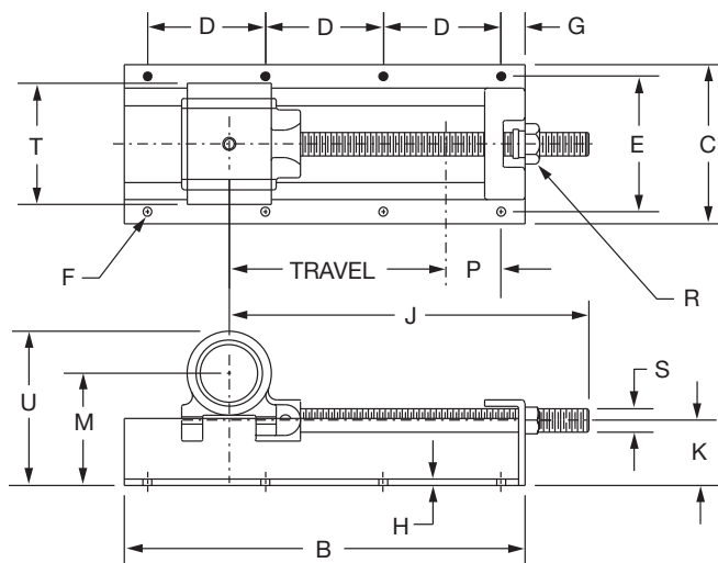
TYPE TUB
