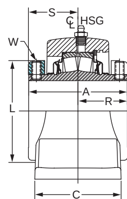
4-7/16 THRU 4-15/16" CONSTRUCTION NON-EXPANSION
