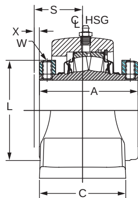
4-7/16 THRU 4-15/16" CONSTRUCTION EXPANSION
