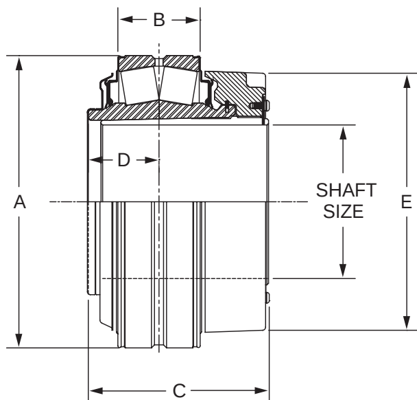
TRIDENT SEAL
