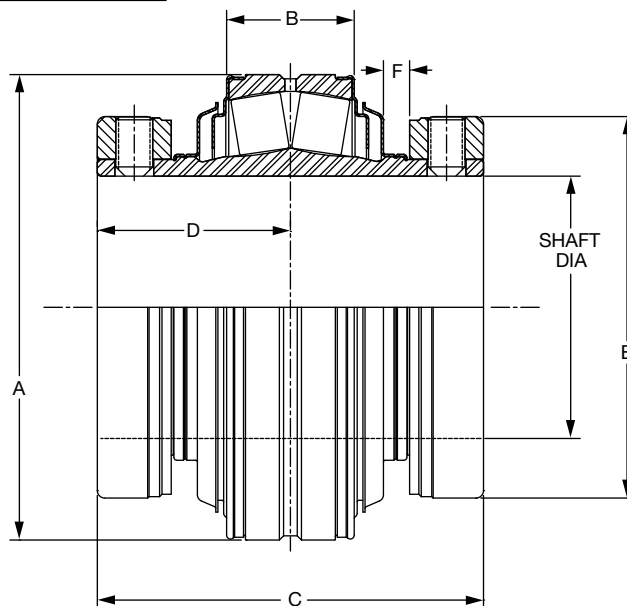
4-7/16 THRU 4-15/16" CONSTRUCTION
