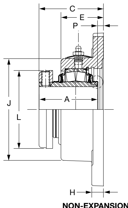
NON-EXPANSION
