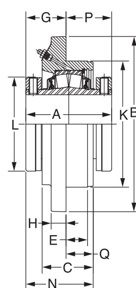
4-7/16 THRU 5" CONSTRUCTION NON-EXPANSION
