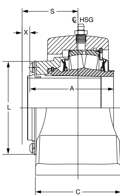
EXPANSION
