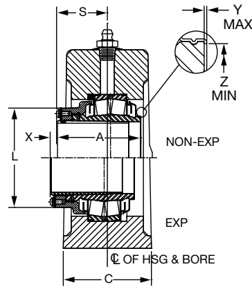
LABYRINTH SEAL
