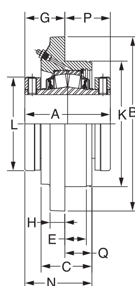
4-7/16 THRU 5" CONSTRUCTION
