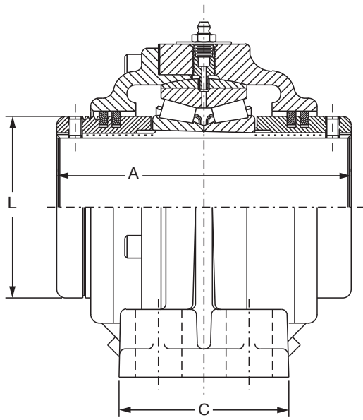
EXPANSION CONSTRUCTION
