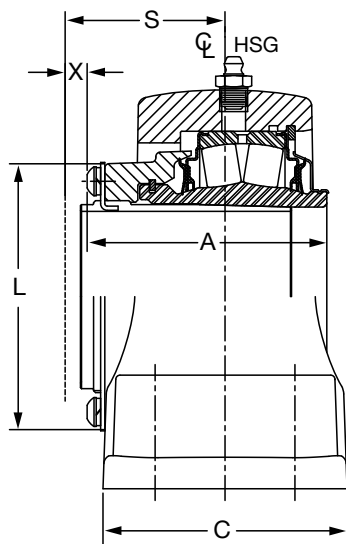
3-11/16" THRU 5" EXPANSION
