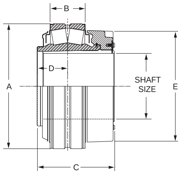
LABYRINTH SEAL
