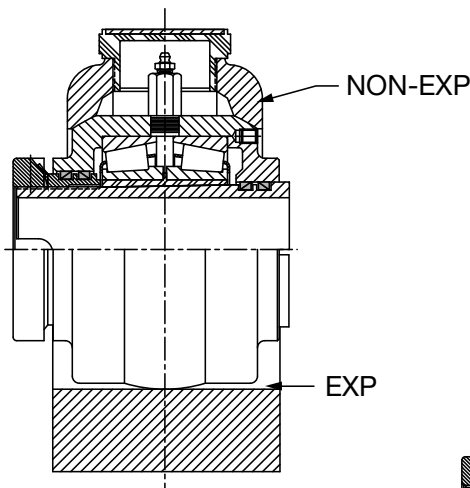
2-3/8" THRU 3-1/2" CONSTRUCTION
