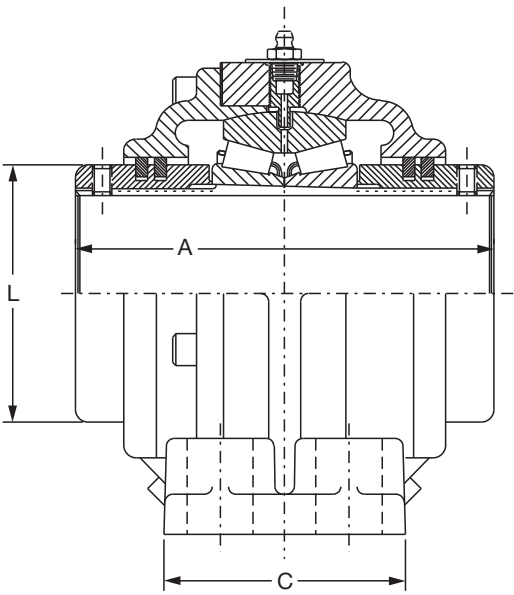
NON-EXPANSION CONSTRUCTION
