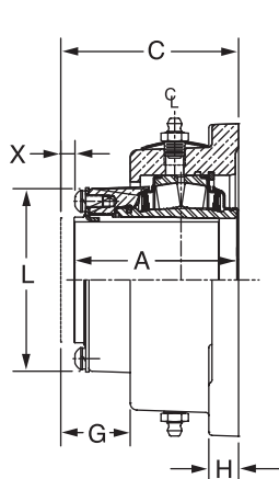
EXPANSION
