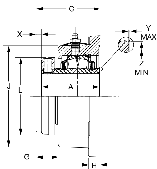
EXPANSION
