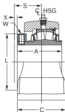
2-7/16 THRU 3-15/16" CONSTRUCTION EXPANSION
