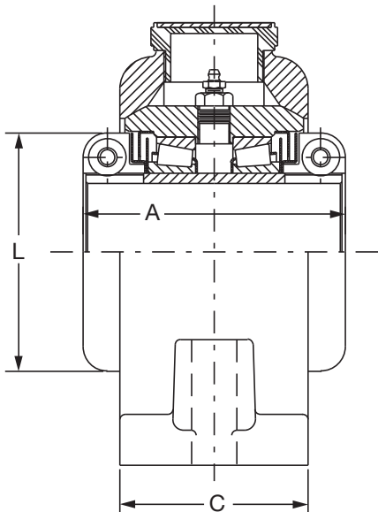
NON-EXPANSION CONSTRUCTION
