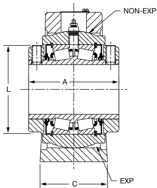
1-3/16" THRU 3" CONSTRUCTION
