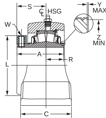
2-7/16 THRU 3-15/16" CONSTRUCTION NON-EXPANSION
