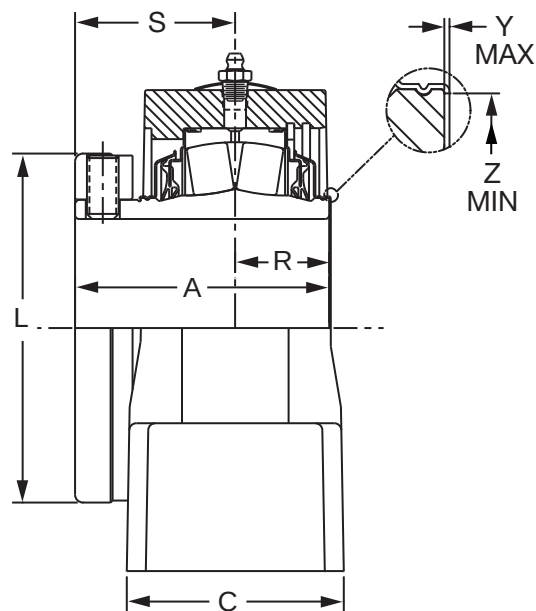
NON-EXPANSION
