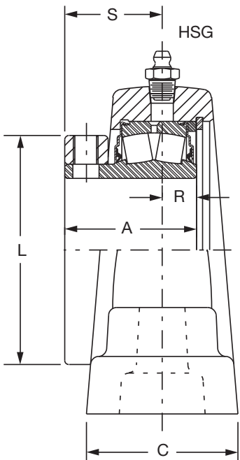
NON-EXPANSION
