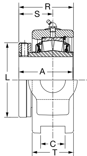
1-3/8 THRU 3-15/16" CONSTRUCTION
