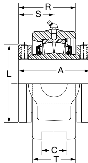
4-7/16 THRU 4-15/16" CONSTRUCTION
