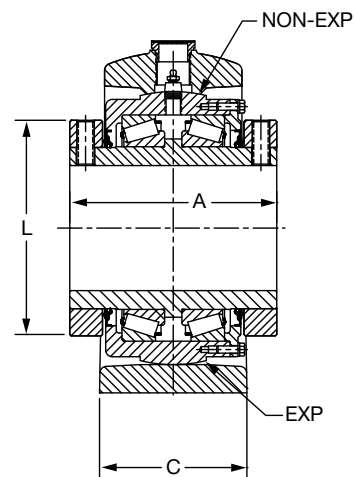
5-7/16" THRU 7" CONSTRUCTION
