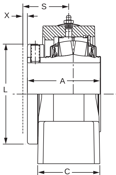
EXPANSION
