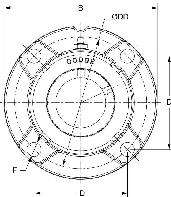
1-11/16" - 3" CONSTRUCTION
