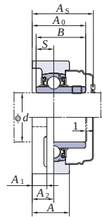
With Pressed Steel Cover
