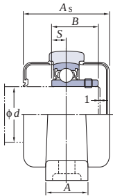
With One Side Sealed Cover
