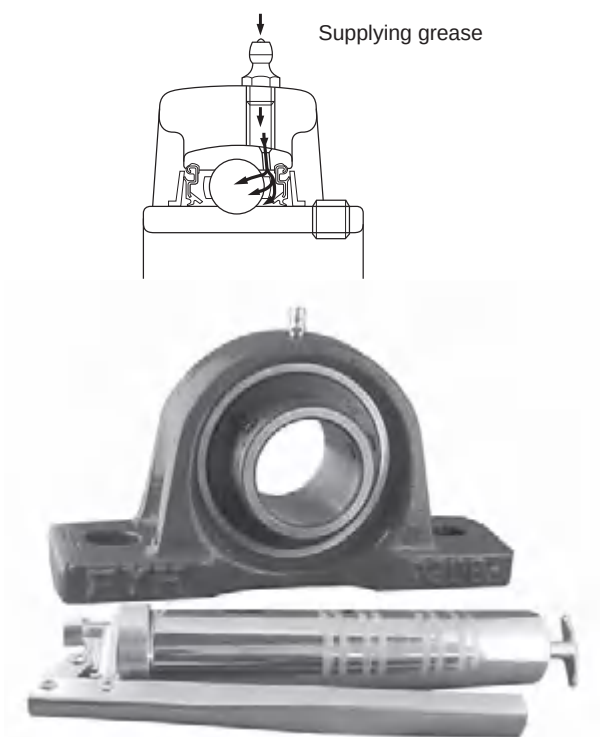
Fig. 14.14 Supplying grease to ball bearing units
