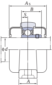
With Through Type Cover
