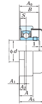
With One Side Sealed Cover
