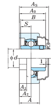
With Pressed Stainless Steel Cover
