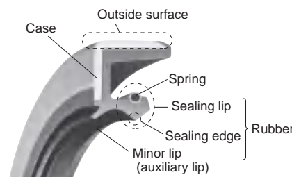
Fig. 14-8 Names of oil seal parts
