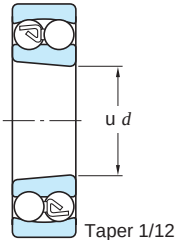
Tapered bore
