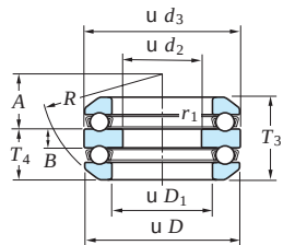
With spherical back faces
