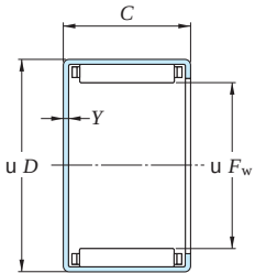
MJ-1, MJH-1
