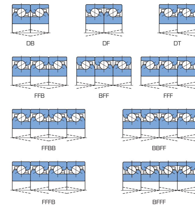
Figure 4.3 Flush Ground Bearing Set Combinations and Combination Marks (For angular contact ball bearings and ball screw support bearings)
