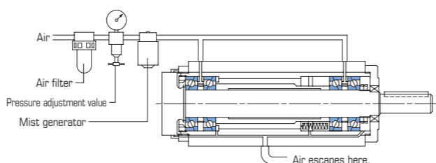
Figure 6.2 Example of Spindle Unit Using Vapor Lubrication
