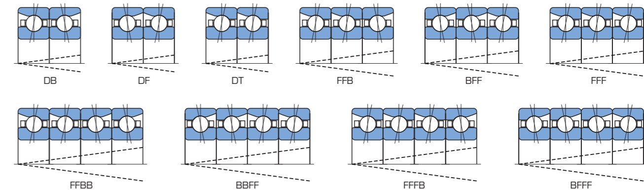
Figure 4.1 Set Combinations and Outer Ring Combination Marks
