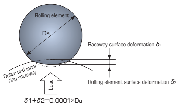
Figure 2.2 Permanent Indentation
