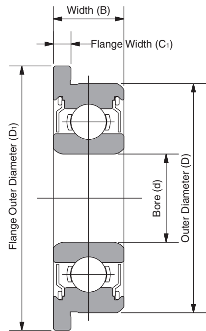
With flange
