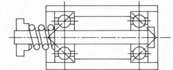
Figure 12-3 Constant pressure preload
