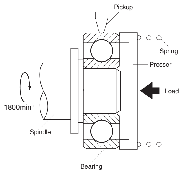
Schematic diagram of detector
