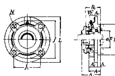
Pressed steel dust cover type
