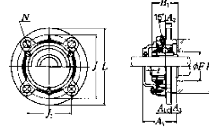
Cast dust cover type
