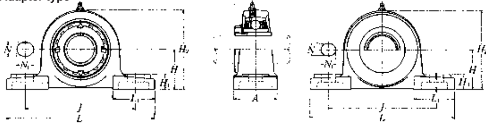
Pressed steel dust cover type Open end Z-UKP...D1 Closed end ZM-UKP...D1
