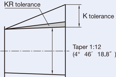
Fig. 7.2 Taper Angle Tolerances
