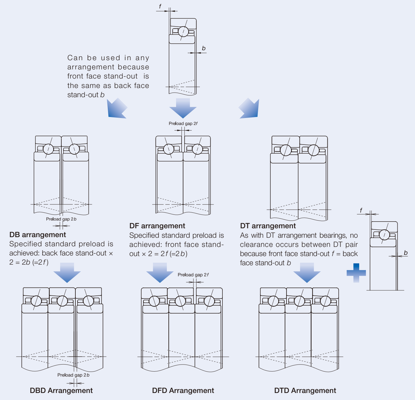
Fig. 3.9 Universal Arrangement
