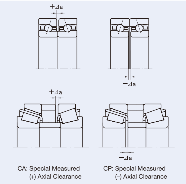
Fig 4.5 Adjustment of Axial Clearance with Spacers
