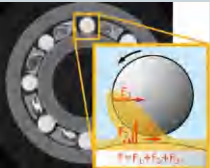
Friction on the bearing's ball surface
