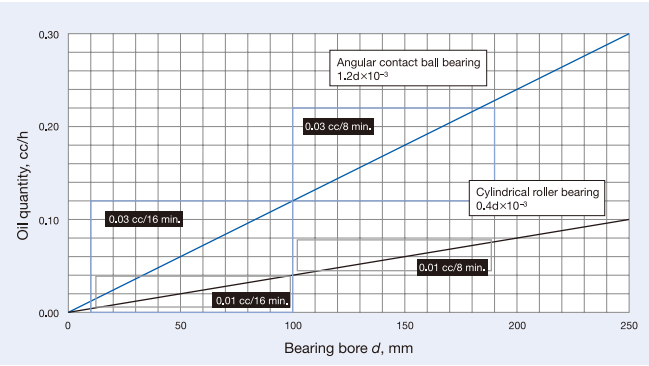
Fig. 6.3 Recommended Oil Quantity by Bearing Bore Size (Minimal Oil Quantity Lubrication)
