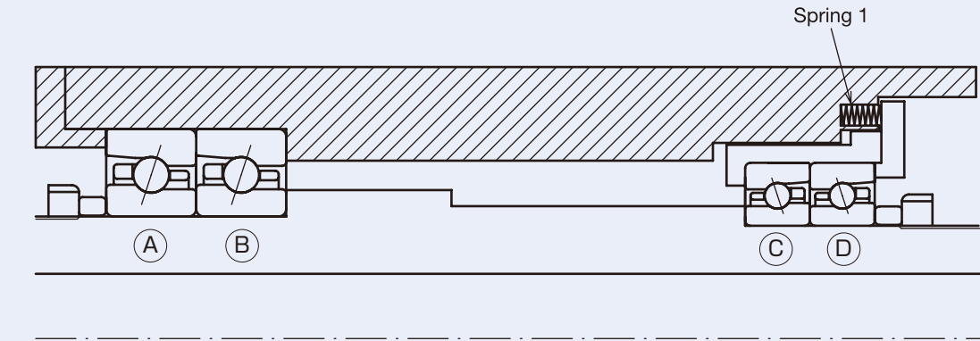
Fig. 4.6 Distribution of Preload in Constant Pressure Preload
