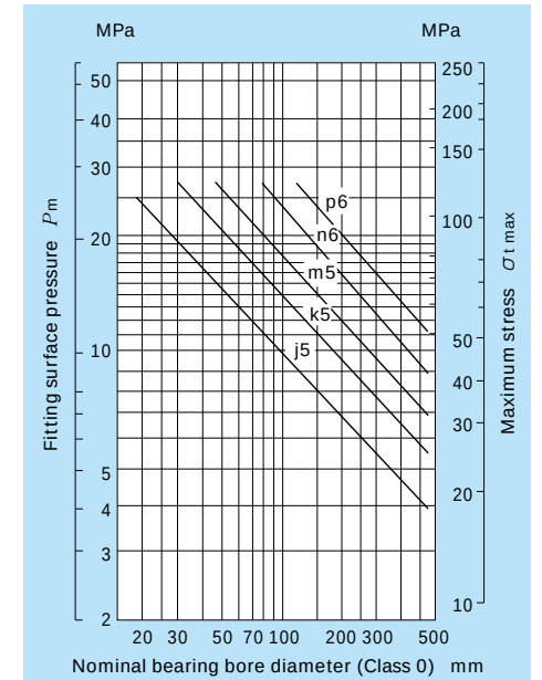
Fig. 17.4.2 Maximum fit interference as it relates to surface pressure P_m and maximum stress \sigma_{t \text{ max}}
