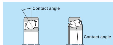
Fig. 1.3 Contact angle
