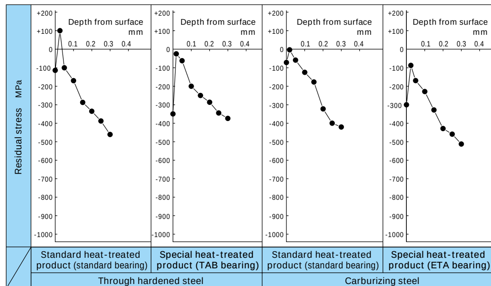
Fig. 13.2 Residual stress within a dent
