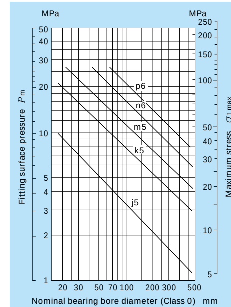
Fig. 17.4.1 Average fit interference as it relates to surface pressure P_m and maximum stress \sigma_{t \text{ max}}
