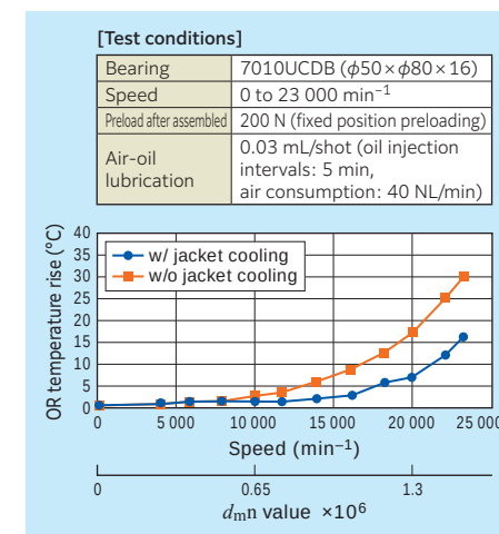
Fig. 9.23 High speed test with air-oil lubrication
