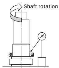
Fig. 6.2 Checking for face runout of inner ring
