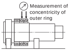
Fig. 6.3 Checking for concentricity of outer ring
