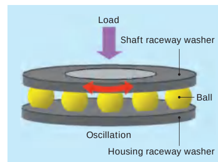
Fig. 13.5 Fretting resistance test (rolling)
