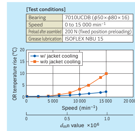
Fig. 9.22 High speed test with grease lubrication
