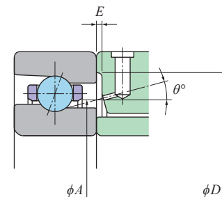
Fig. 7.5 BNT and HTA types
