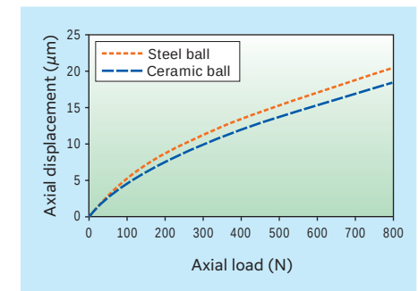
Fig. 9.20 Axial rigidity diagram
