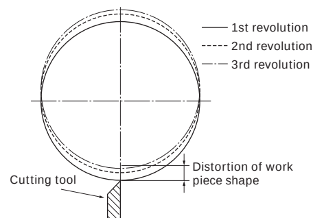
Fig. 2.4 Model of cutting operation
