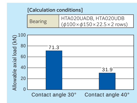
Fig. 11.4 Comparison of allowable axial load
