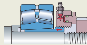
HMV ..E nut and special stop nut for driving in a withdrawal sleeve.
