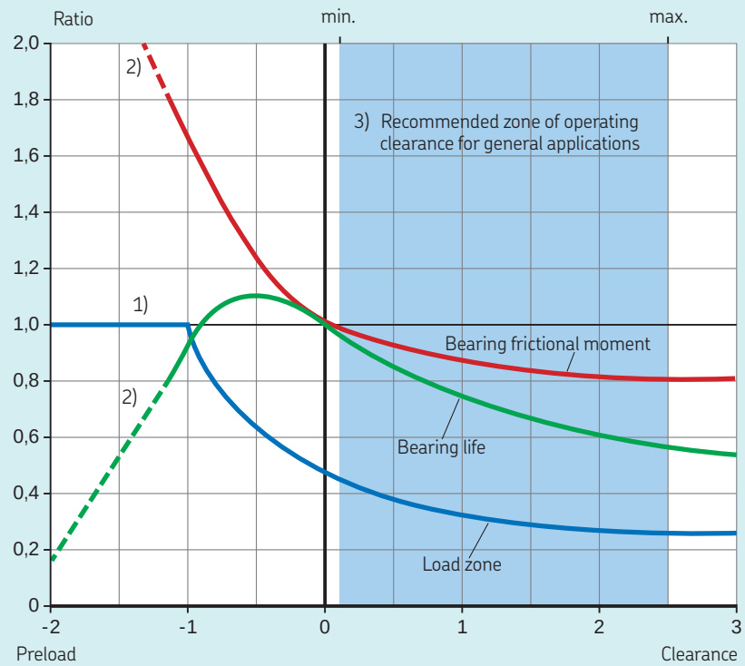
Operational clearance or preload versus main operational criteria
