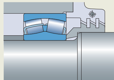
External labyrinth seal, with inclined passages
