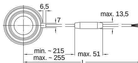
BMB ... 008A (Free cable end)
