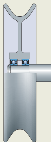
Traditional rope sheave used in paper machines
