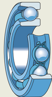
Bearing with filling slots
