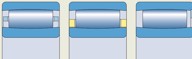
Bearing with a roller centred cage
