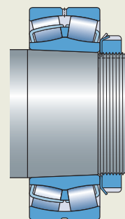
Fig. 3 Bearing with a tapered bore mounted on a tapered seat
