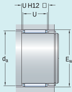
Abutment dimensions for needle roller and cage assemblies
