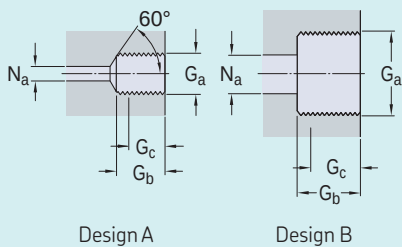
Design and recommended dimensions for threaded holes for connecting oil supply
