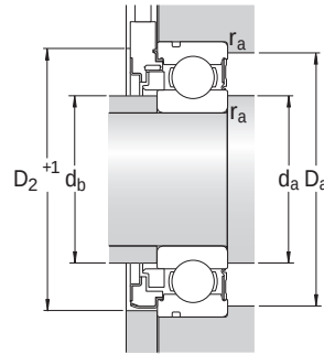
BMB BMO Bore diameter of end cover \geq D_2 + 1 \text{ mm}
