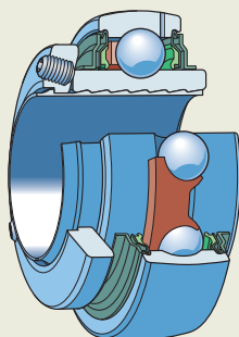
Bearing in the YSP 2 series
