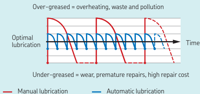
Relubrication method and impact on performance
