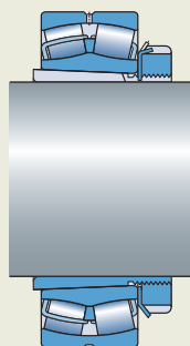
Fig. 2 Bearing with a tapered bore mounted on a plain shaft with an adapter sleeve
