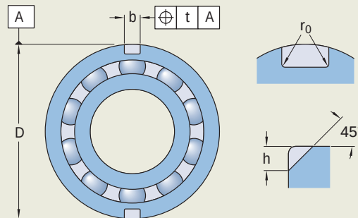
Bearing with additional anti-rotation slots in the outer ring
