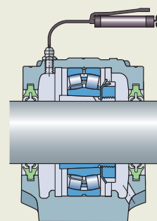
Relubrication from the side
