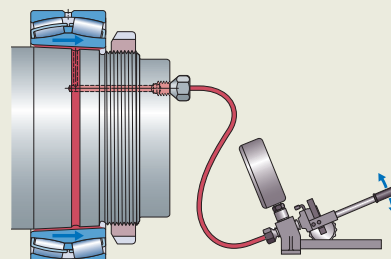
Dismounting with aid of oil injection – a stop is provided
