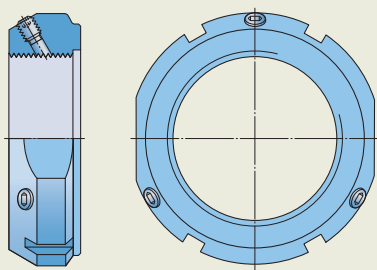
KMT lock nut with two opposed flats
