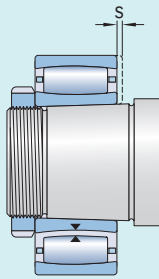
Drive-up data for CARB bearings with a tapered bore
