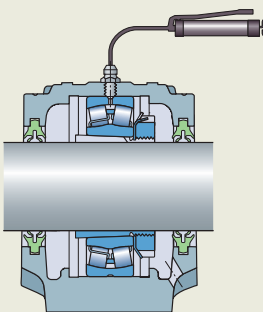
Relubrication in the centre
