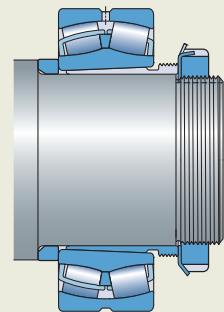
Withdrawal sleeve on a stepped shaft
