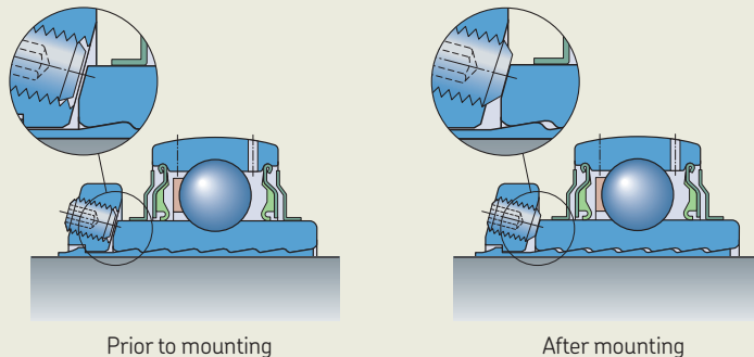
SKF ConCentra locking technology
