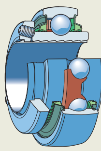
Bearing in the YSPAG 2 series
