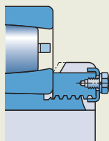
E (with an HME nut)
