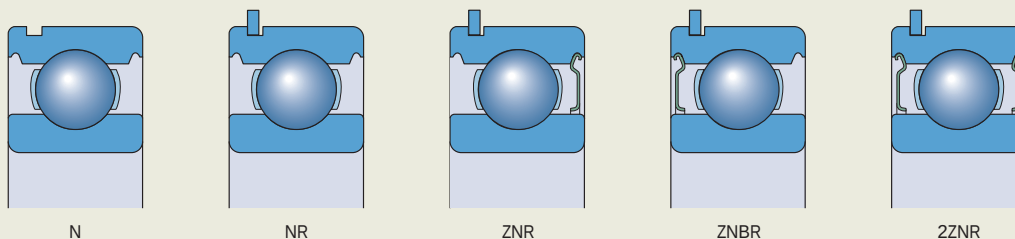
Bearing variants with a snap ring groove
