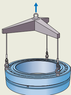
Eye bolts in bearing ring to ease lifting
