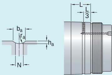
Recommended dimensions for oil supply ducts and distribution grooves
