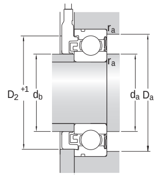
BMD Bore diameter of end cover \geq D_2 + 1 \text{ mm}
