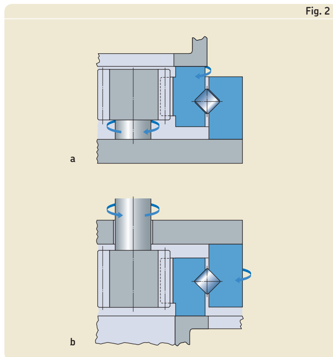
Pinion drive arrangements
